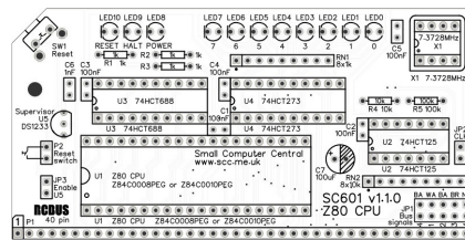
SC601 - Z80 CPU
