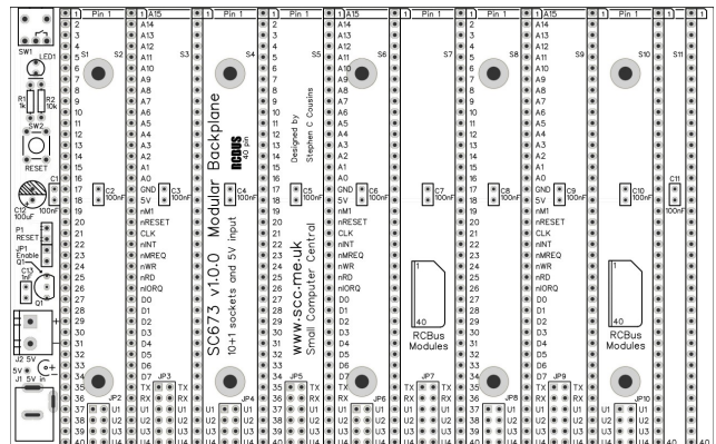
SC673 - Backplane 10+1 with 5 volt power input
