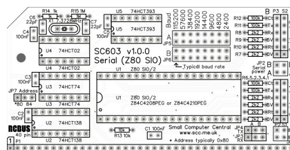
SC603 - Z80 SIO/2 dual serial
