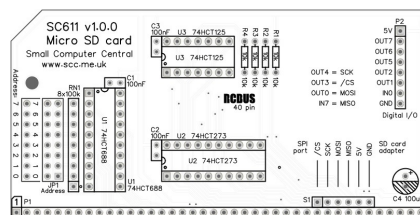
SC611 - MicroSD card storage with adapter
