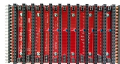
SC710 - Backplane plus SC703 PSU
