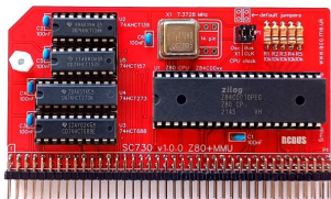
SC730 - Z80 CPU plus MMU
