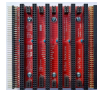
SC702 - Backplane plus SC703 PSU
